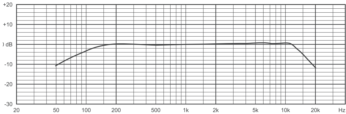
Frequency response curve \pm 2.5 dB
