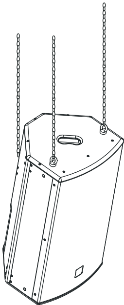
Suspension using M10 shoulder eyebolts.
