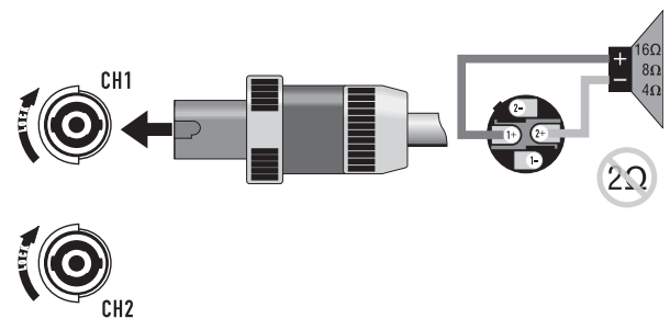
Mode Mono pont – Figure 31 –
