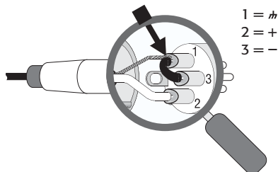
XLR unbalanced Jumper pin 1 to pin 3 – Abbildung 26 –
