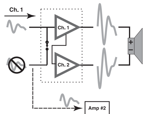
Channel 2 Can Be Used to Daisy-chain to Other Amplifiers. – Figure 22 –
