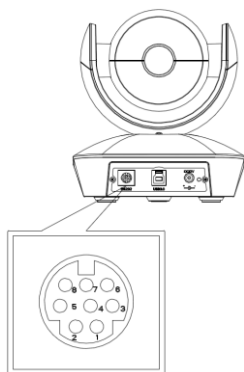
VISCA IN &RS485 Connection
