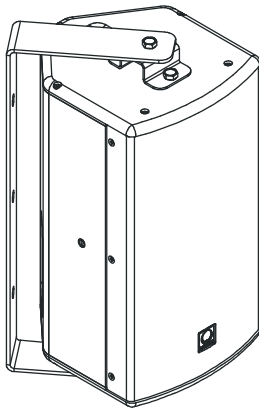
NuQ62-SB swivel bracket for surface mounting
