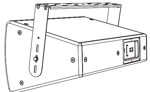
Horizontal Mounting
